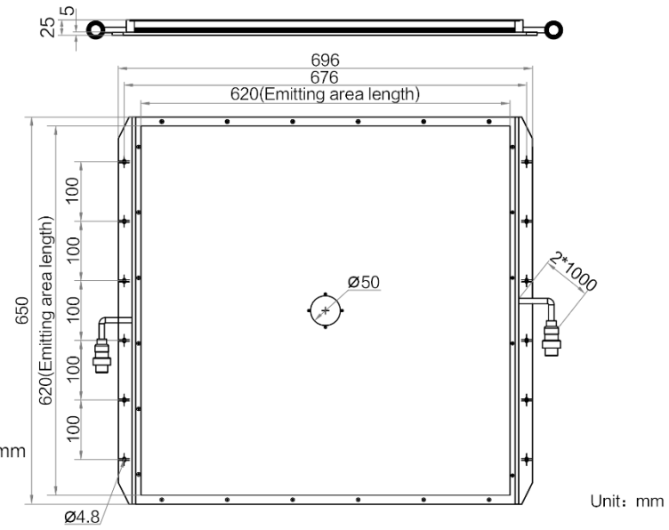
MV-LBES-H-620-620-W
