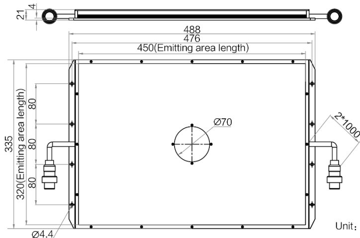
MV-LBES-H-450-320-W
