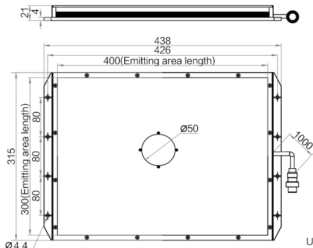
MV-LBES-H-400-300-W
