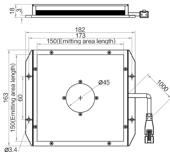
MV-LBES-H-150-150-W
