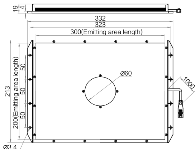
MV-LBES-H-300-200-W
