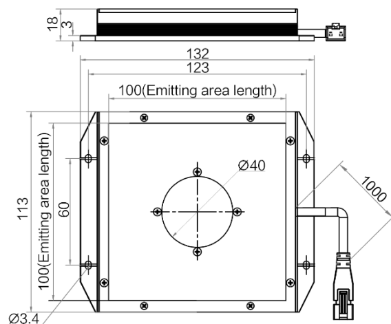
MV-LBES-H-100-100-W
