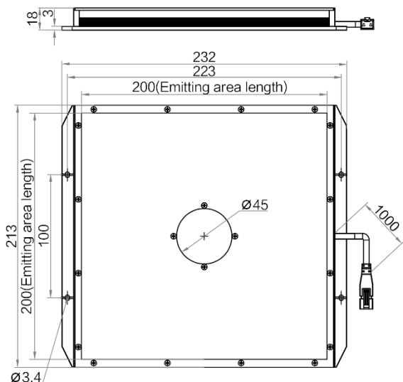
MV-LBES-H-200-200-W
