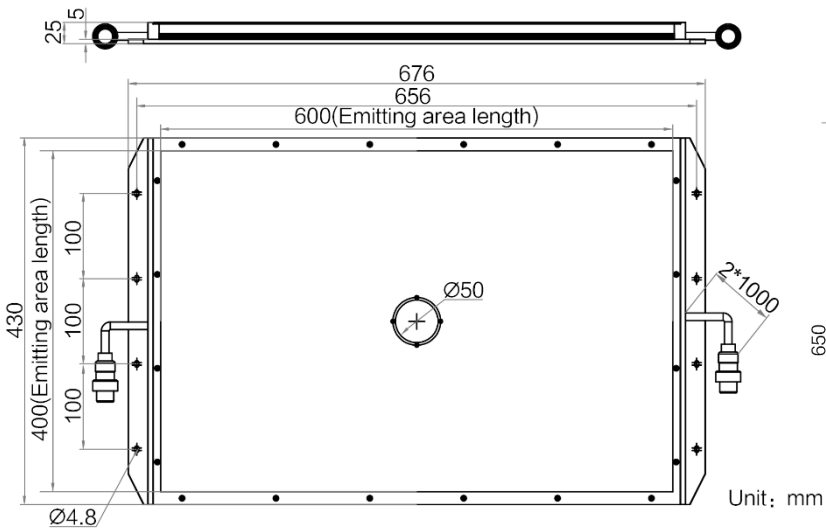
MV-LBES-H-600-400-W
