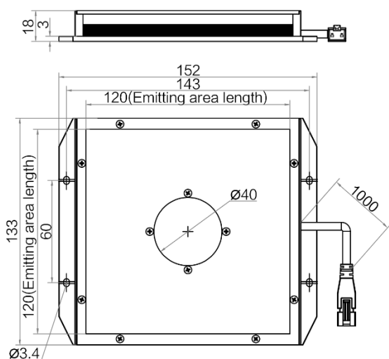
MV-LBES-H-120-120-W
