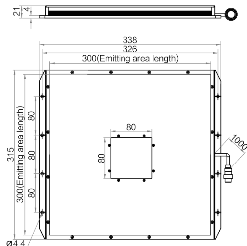
MV-LBES-H-300-300-W
