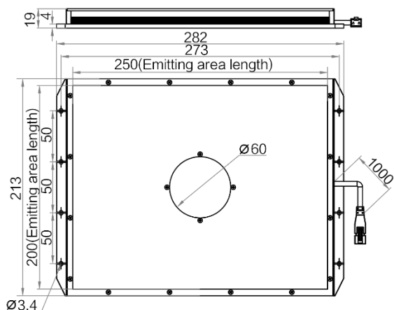
MV-LBES-H-250-200-W
