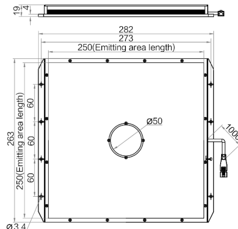
MV-LBES-H-250-250-W/R
